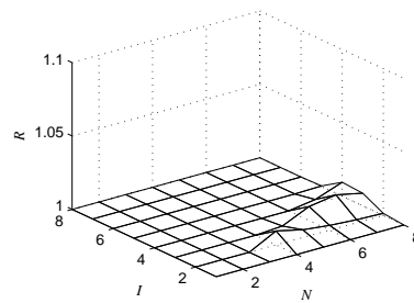
(e) N contenders in a clique with I dependent interferers, a = 0.4 .
